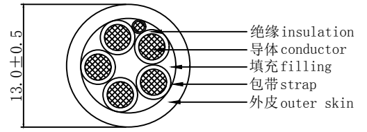
充电枪线缆: 5X2.5mm 2 +1X0.5mm 2 黑色外皮 Charging gun cable: 5X2.5mm 2 +1X0.5mm 2 black
