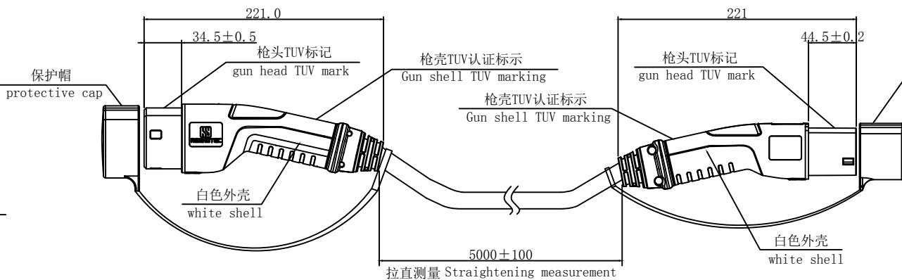
16A车辆端插头7POS 16A Vehicle end plug 7pos
