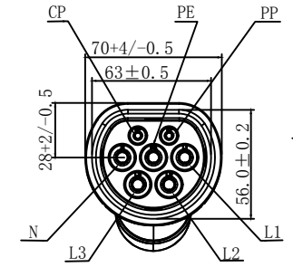
16A车辆端插头7POS 16A Vehicle end plug 7pos
